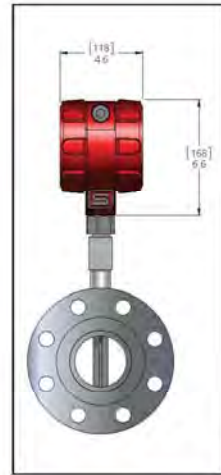
240i Remote Inline Junction Box—Side (Outlet View)
